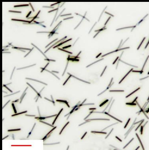
Silver Nanowires, Lot: ST512 Scale bar is 10 \mu m
