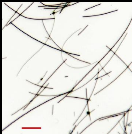
Silver Nanowires, Lot: ST475 Scale bar is 20 \mu m
